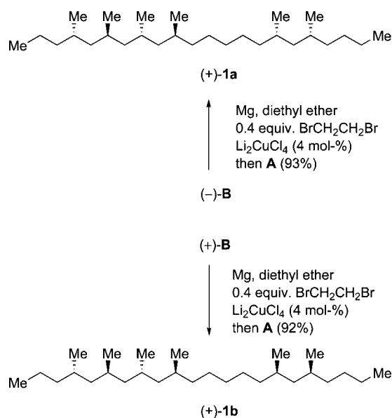
Scheme 5. Fragment coupling through Cu-catalyzed \text{sp}^3\text{--sp}^3 cross coupling. Synthesis of (+)- 1a and (+)- 1b .
